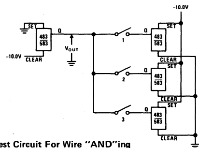
FIGURE 7. Test Circuit For Wire "AND"ing
