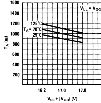
Guaranteed Access Time vs Supply Voltage
