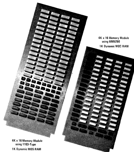
FIGURE 7. 1103-Type and MM5260 Modules. The 1103 memory module utilizes NH0026 level translators in place of 36 DM74451 and NH0027 elements.
