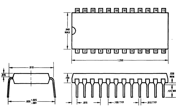
24-Pin Molded Dual-In-Line Package (N)
