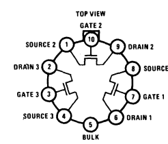
NOTE: Pin 5 connected to case and device bulk. Drain and Source may be interchanged. MM455, MM555
