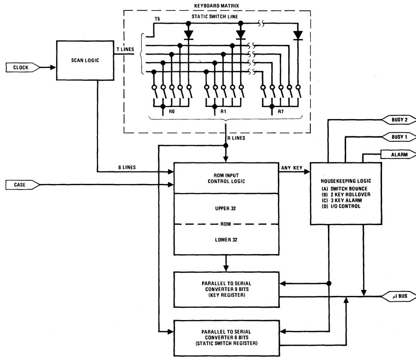
FIGURE 2. MM5704 KI Block Diagram
