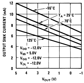
Output Sink Current vs Voltage
