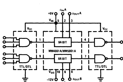
MM4001A/MM5001A TTL/MOS Interface
