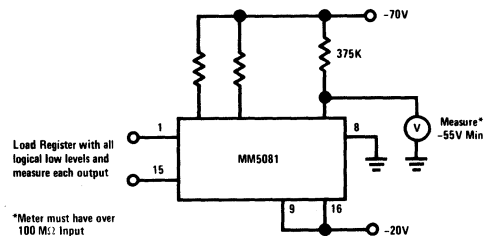
Leakage Test
