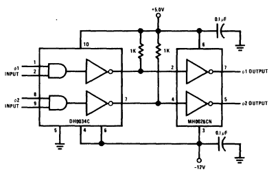
DC Coupled MOS Clock Driver
