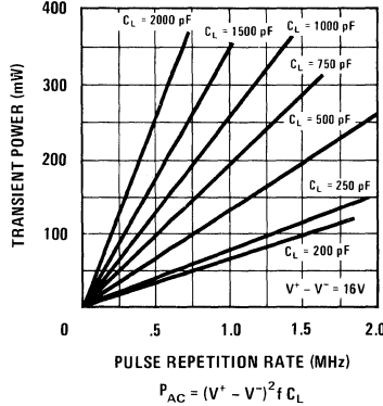
Transient Power vs Rep. Rate
