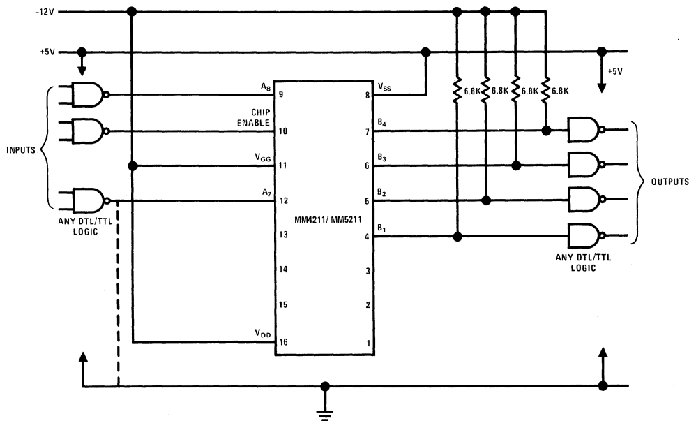
256 x 4 Bit ROM Showing TTL Interface
