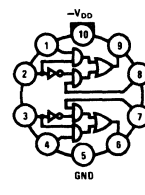
MM482/MM582 dual digital multiplex switch
