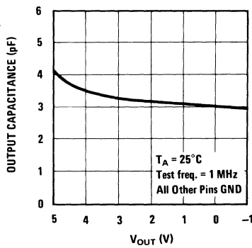
Typical Tri-State Data Output Capacitance vs Voltage
