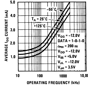
Power Supply Current vs Operating Frequency
