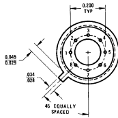
8-Lead Metal Can Package (H)
