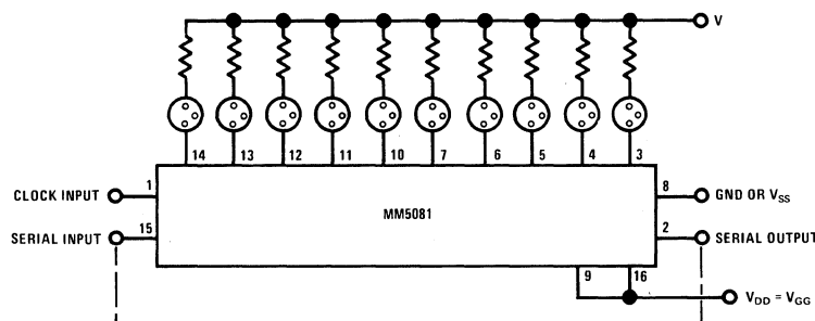
FIGURE 1. Block Diagram
