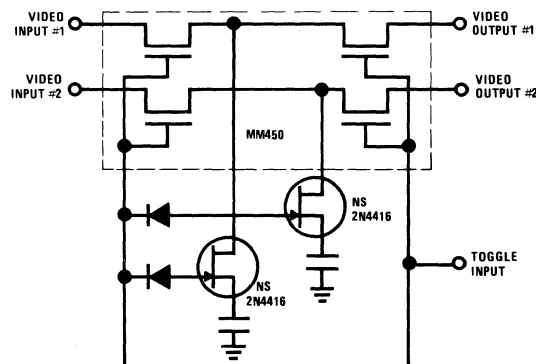
DPST High-Frequency Switch
