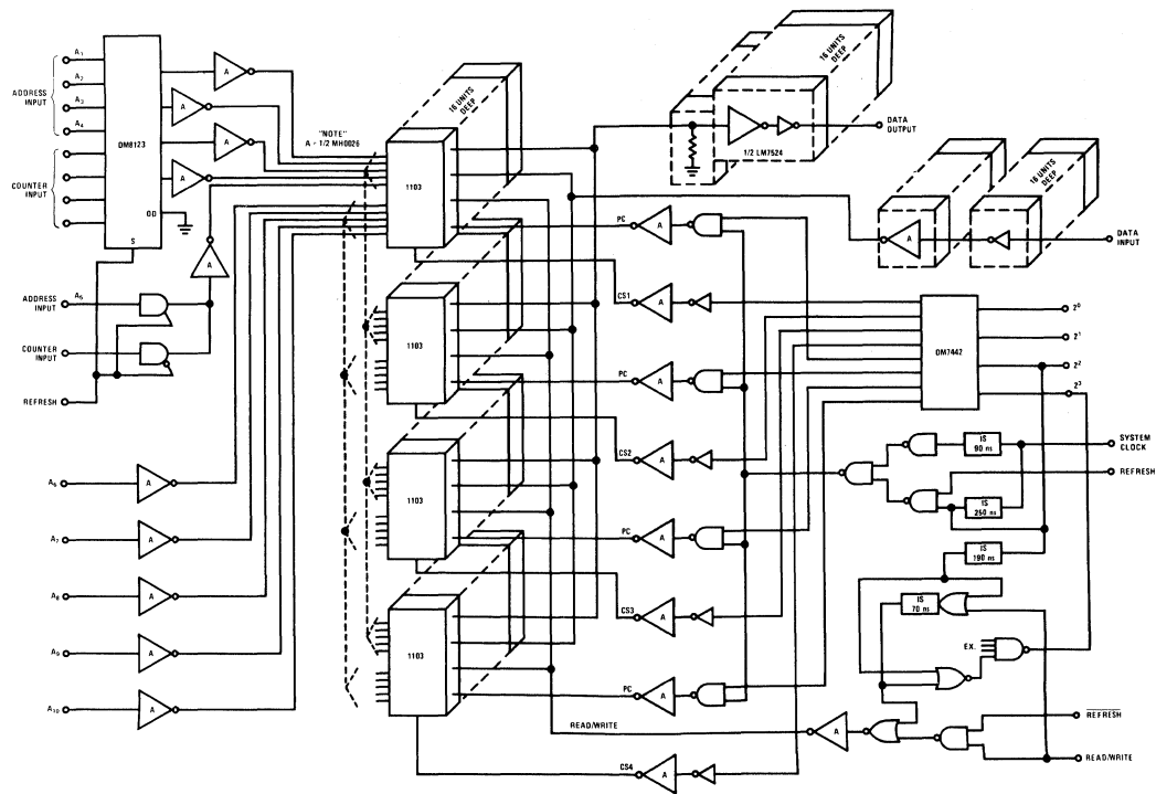
FIGURE 5. Main Memory Module with Conventional 1103-Type MOS RAMs
