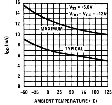
Power Supply Current vs Ambient Temperature
