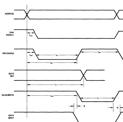
FIGURE 4. MM5260 Timing Diagram
