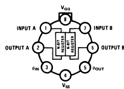
Standard Connection
