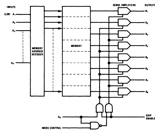
256 x 8 Bit ROM Showing TTL Interface
