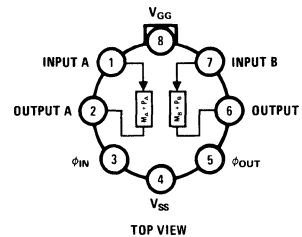
FIGURE 1. Dual Shift Registers
