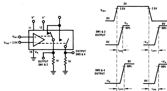
Differential Input
