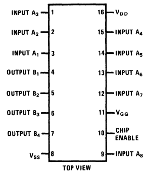
Dual-In-Line Package
