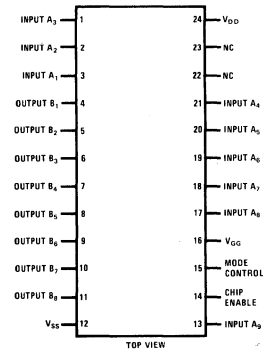
Dual-In-Line Package
