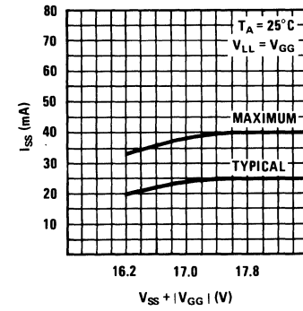
Power Supply Current vs Voltage
