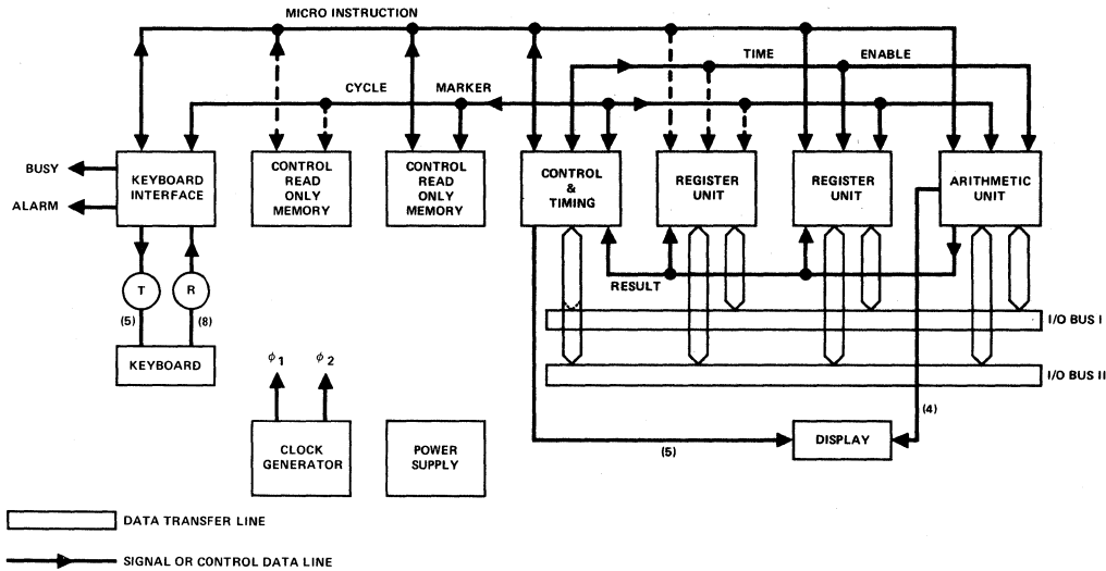
FIGURE 2. MAPS Block Diagram
