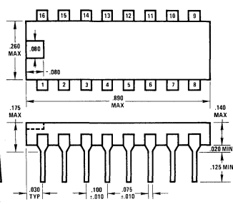
16-Pin Molded Dual-In-Line Package (N)
