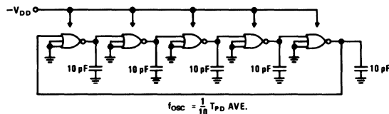
FIGURE 1. Ring Oscillator for Measuring Average Propagation Delay
