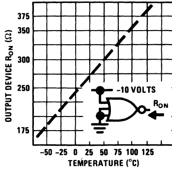
Output Device R_{ON} vs Temperature
