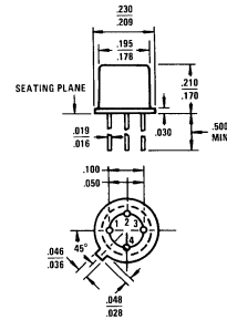
4-Lead Metal Can Package (H)
