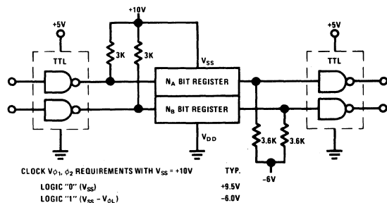
FIGURE 2 – TTL/MOS Interfaces
