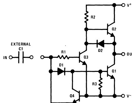
FIGURE 3. Simplified MH0026
