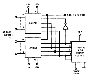
16-Channel Commutator
