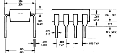
8-Pin Molded Mini-Dual-In-Line Package (N)
