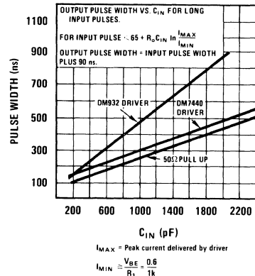
Output P.W. Controlled by C IN
