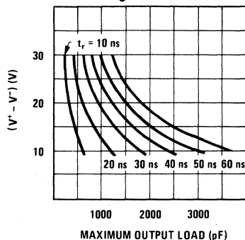
FIGURE 1. Output Load vs Voltage Swing
