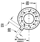
10-Lead Metal Can Package (H)
