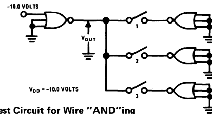
FIGURE 4. Test Circuit for Wire "AND"ing
