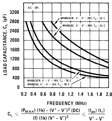
Maximum Load Capacitance
