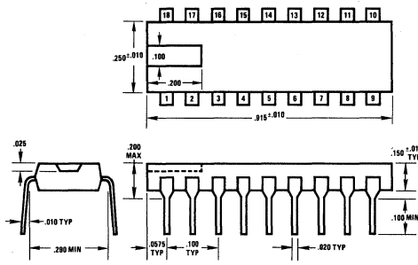
18-Pin Molded Dual-In-Line Package (N)
