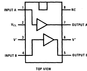
Dual-In-Line Package
