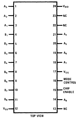
Dual-In-Line Package
