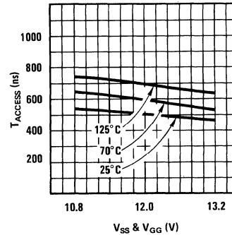
Typical Access Time vs Supply Voltages
