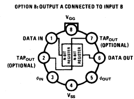
Optional Connections
