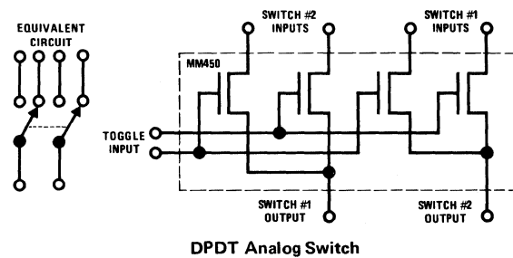
DPDT Analog Switch
