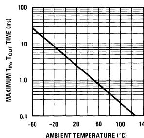
FIGURE 3. Maximum Partial Bit Time vs Ambient Temperature
