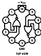
MM480/MM580 dual 3-input NOR gate
