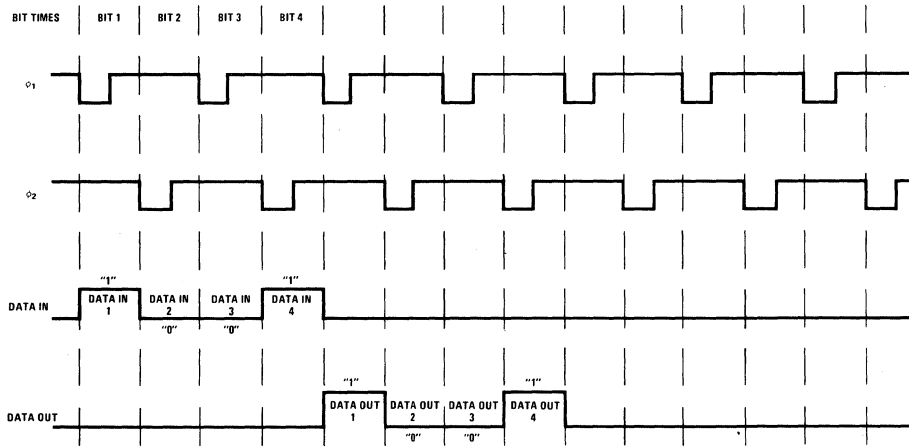
Multiplexed 4-Bit MOS Shift Register
