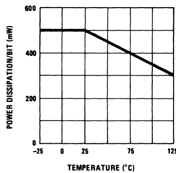
Maximum Package Power Dissipation
