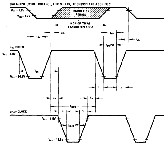
For Writing Data
