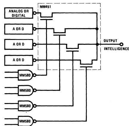
4-Channel Multiplexer*
