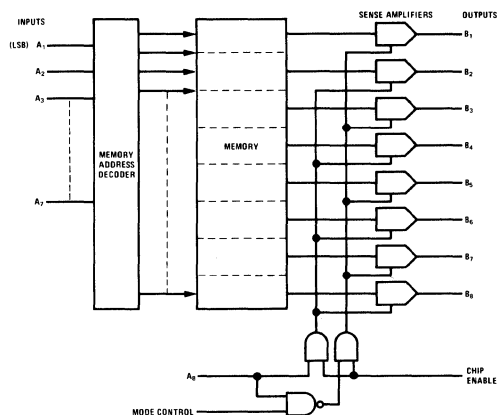
128x8 Bit ROM Showing TTL Interface
