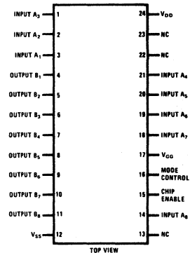
Dual-In-Line Package
