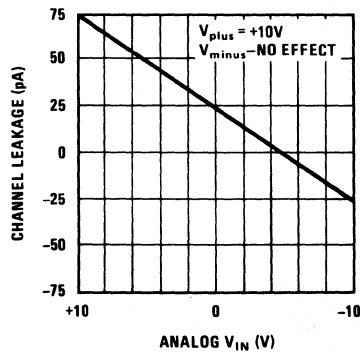
Leakage vs V_{IN} (Channel "OFF")
