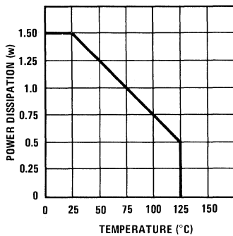
FIGURE 2. Maximum Power Dissipation
