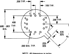
12-Lead Metal Can Package (G)
