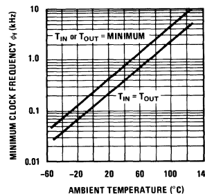
FIGURE 4. Minimum Clock Frequency vs Ambient Temperature
