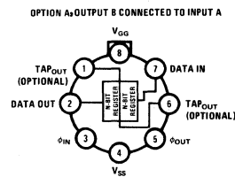
Optional Connections
